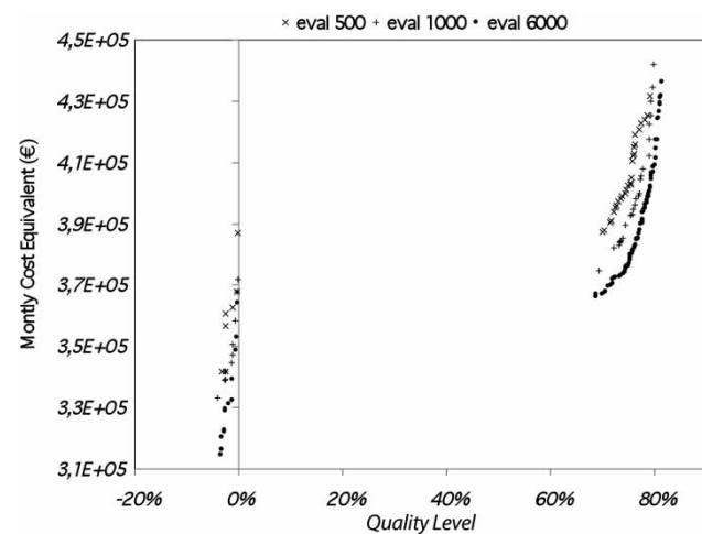
Figure 7 | Pareto fronts considering two objectives (monthly cost and ammonia quality levels) for different number of WQM evaluations (500, 1,000 and 6,000) for the January 2015 Muga scenario.
